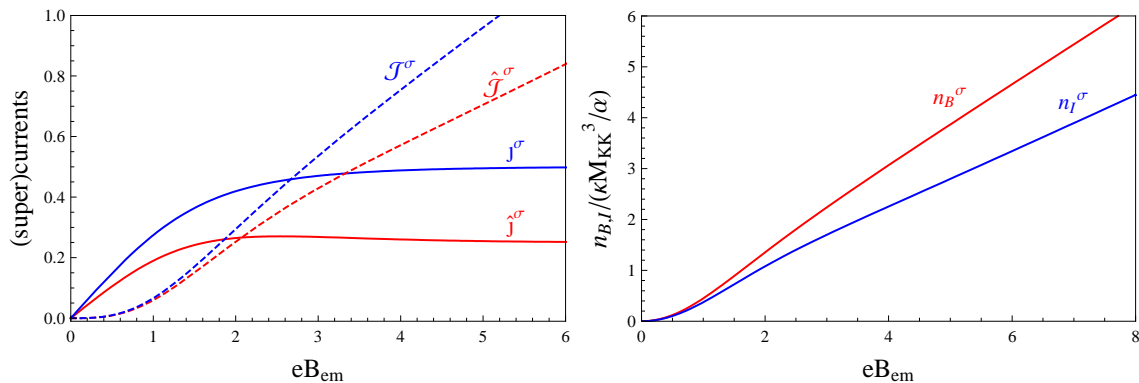
Figure 2. Left panel: Meson supercurrents \hat{j}^\sigma (red solid) and j^\sigma (blue solid) and normal currents \hat{J}^\sigma (red dashed) and J^\sigma (blue dashed) as a function of the dimensionless magnetic field eB_{em} in the sigma phase. The units are M_{KK}/\alpha for \hat{j}^\sigma , j^\sigma and \kappa M_{KK}^3/\alpha for \hat{J}^\sigma , J^\sigma . Right panel: baryon and isospin number densities as a function of the dimensionless magnetic field in the sigma phase. The analytical expressions for the functions are given in eqs. (4.15), (4.18), and (4.33). We have fixed \mu_B = 2\mu_I = M_{KK}\alpha . In the (charged) pion phase, all currents as well as the baryon density vanish due to the Meissner effect; the isospin density is given by the simple expression (4.36b).
